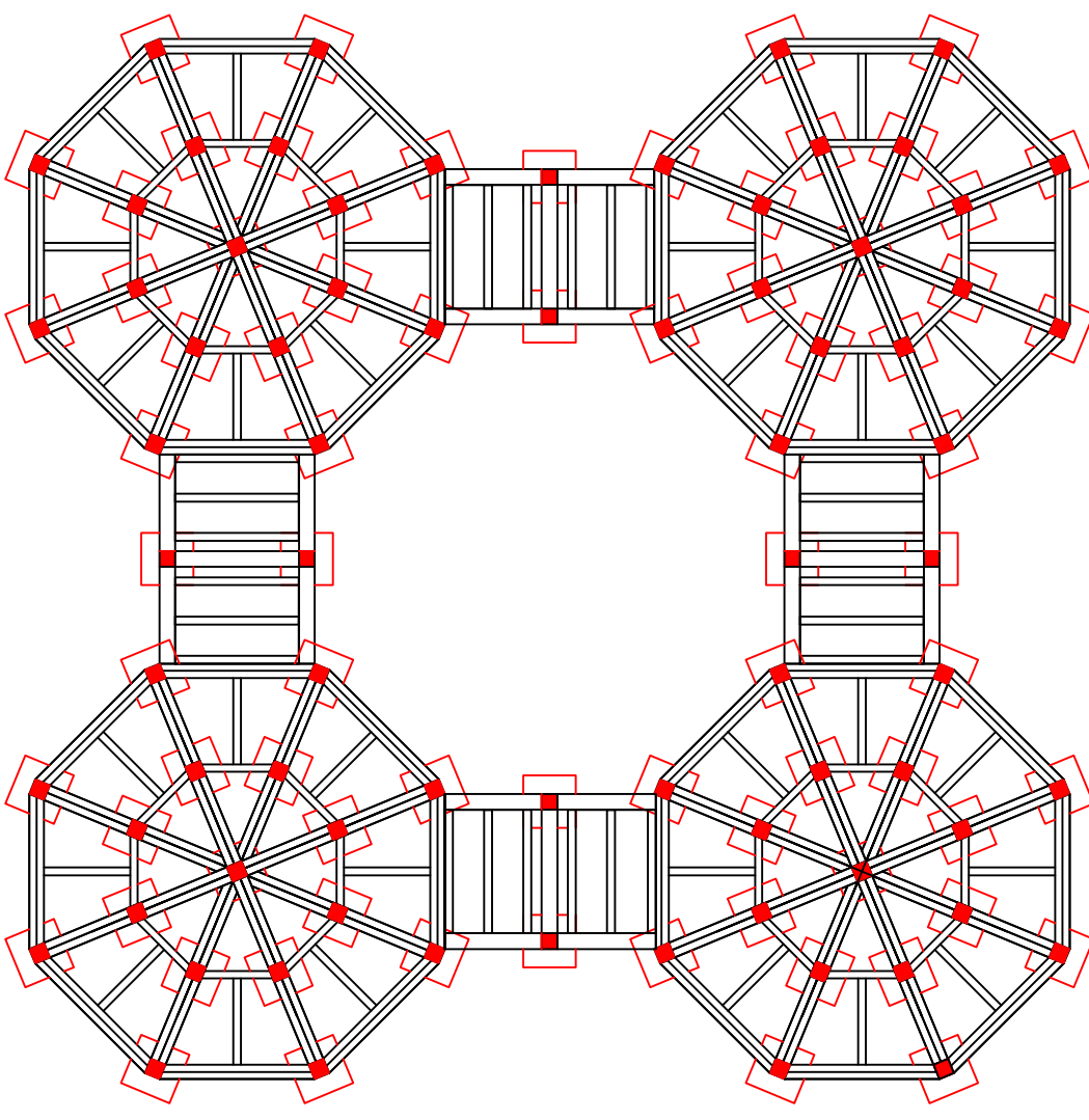
Base plan
