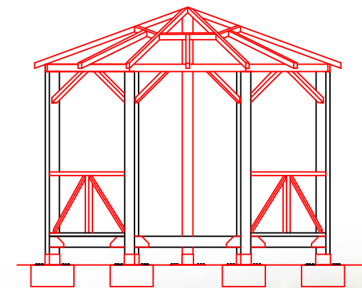
The gazebo construction divided in units (Side view)
