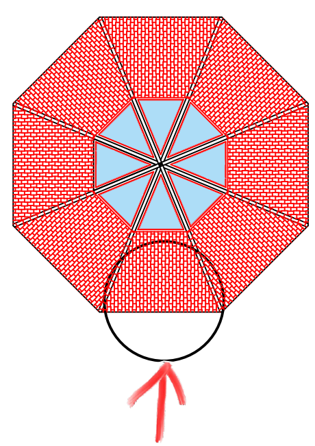
Roof plan (Fifth facade)
